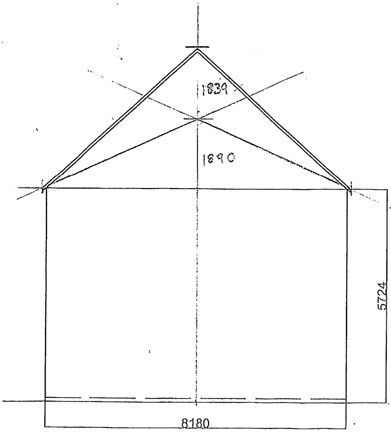
South Elevation
