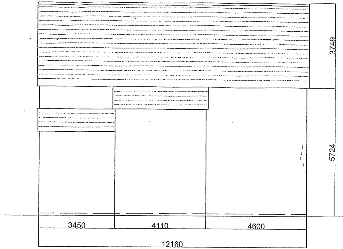
Rear Elevation
