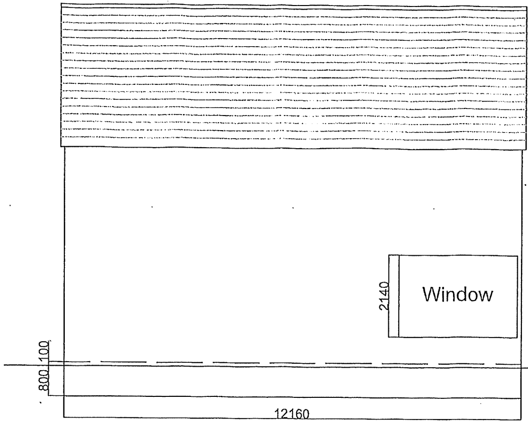
Front Elevation
